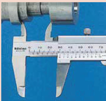
ID measurement
